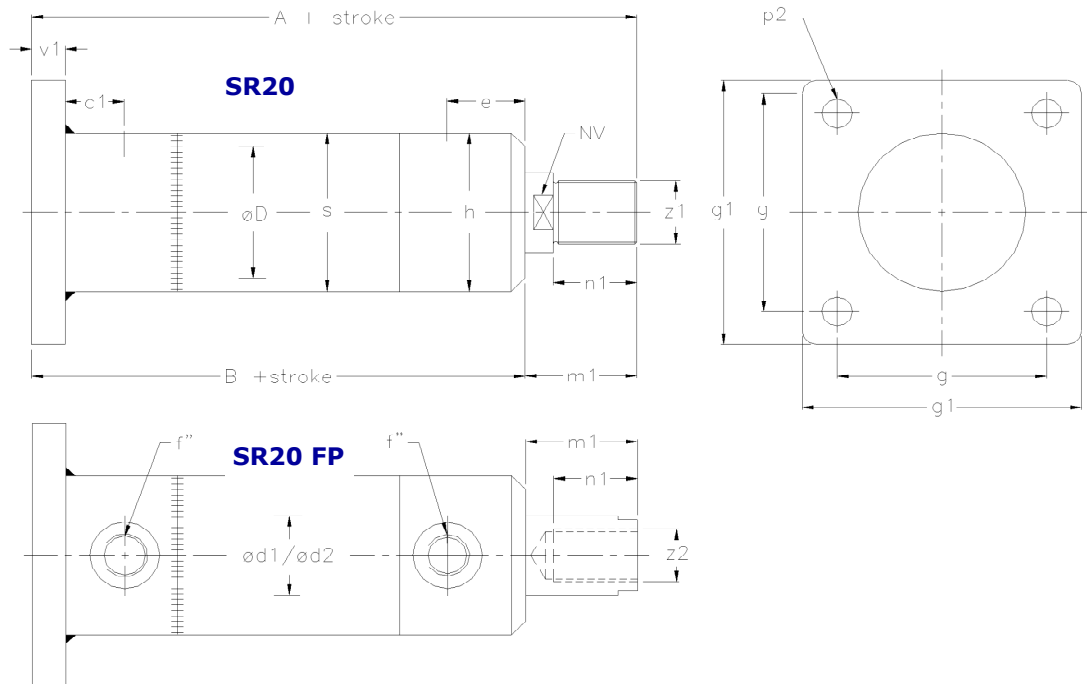
Dimension table
